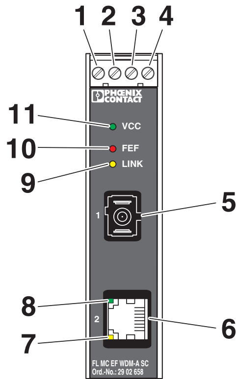
Schematic diagram
